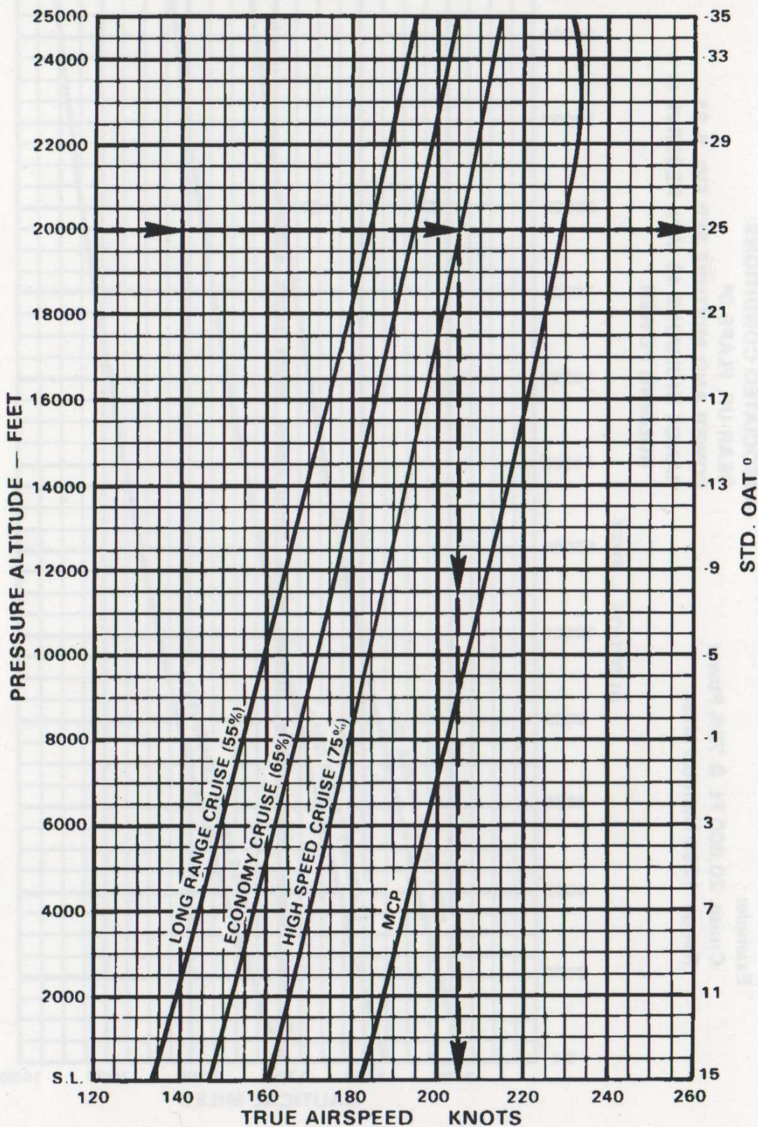
CRUISE SPEED VS. ALTITUDE
